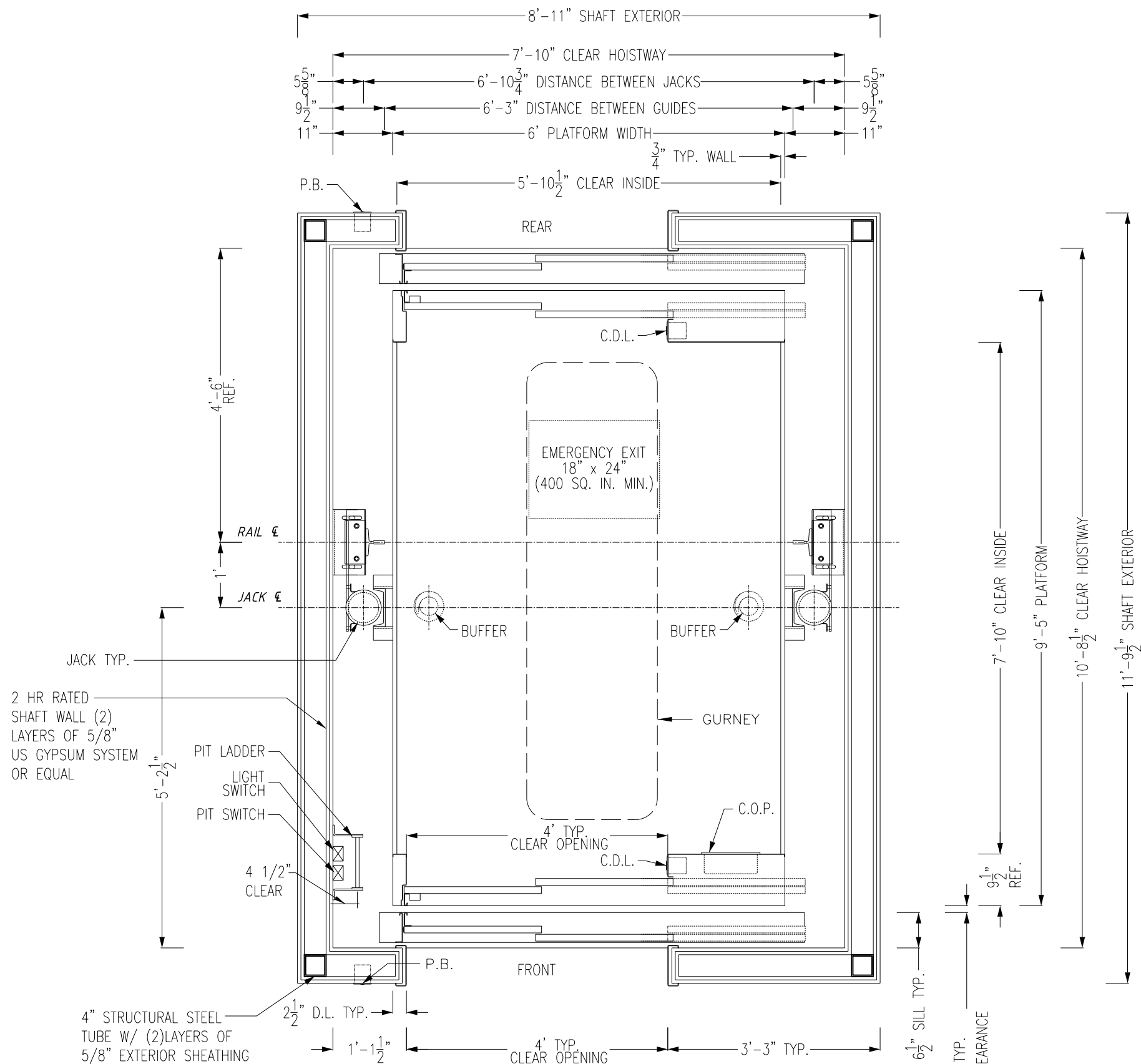
HOISTWAY PLAN
